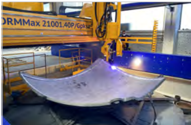
Dome & petal processing
