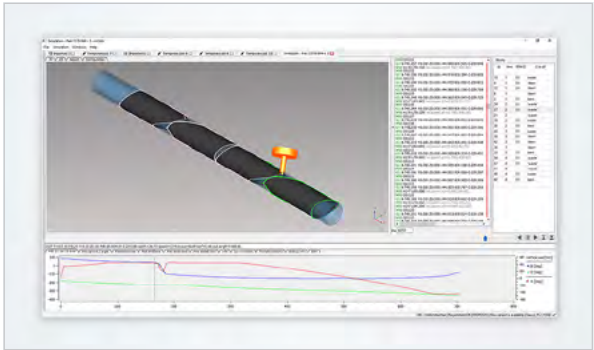
Simulation of the cutting process
