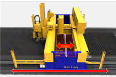
Double-beam gantry
