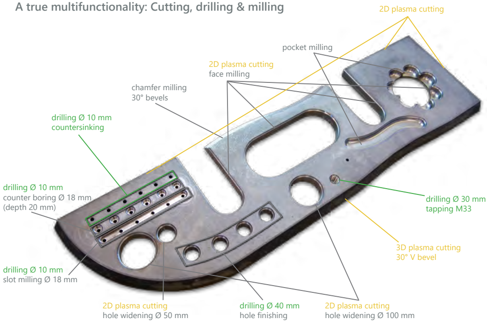
A true multifunctionality: Cutting, drilling & milling
